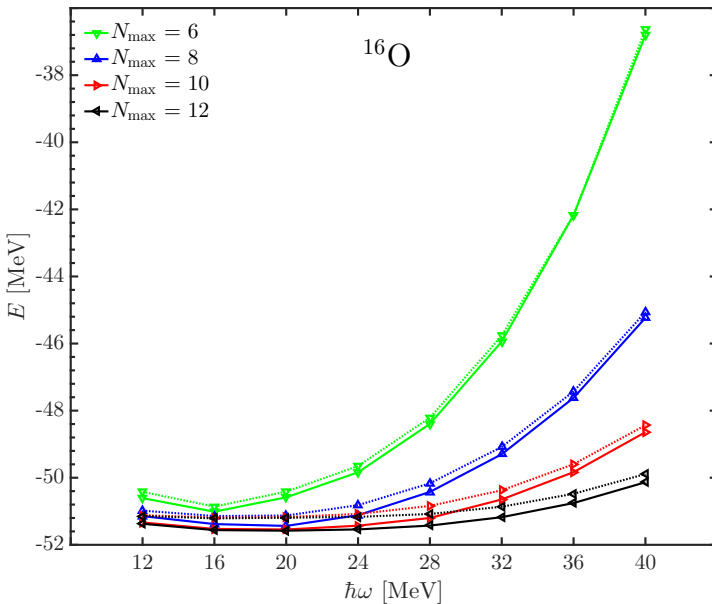
Fig. 1. The HF (full lines) and the NAT (dotted lines) ground-state energies, E = \langle \text{HF} | \hat{H} | \text{HF} \rangle and E = \langle \text{NAT} | \hat{H} | \text{NAT} \rangle , calculated for various N_{\max} , plotted versus the HO frequency.
