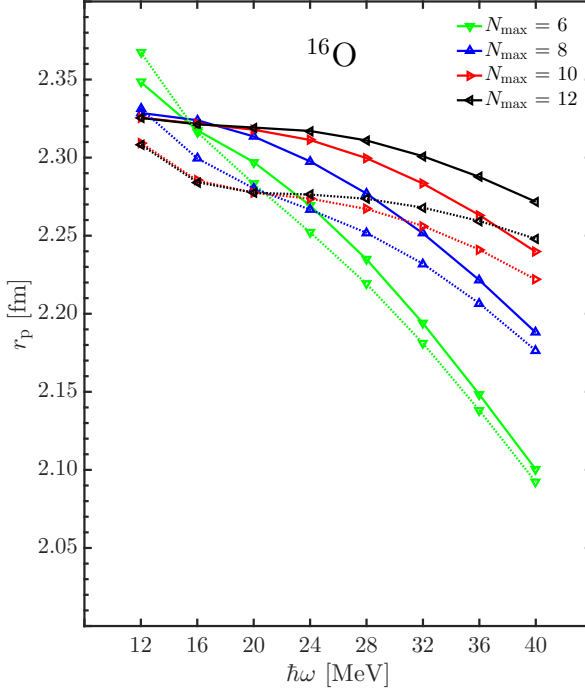
Fig. 2. The proton point-like radii r_p = \sqrt{\langle \text{HF} | r^2 | \text{HF} \rangle} (full lines) and r_p = \sqrt{\langle \text{NAT} | r^2 | \text{NAT} \rangle} (dotted lines), calculated for different N_{\text{max}} , plotted versus the HO frequency.
