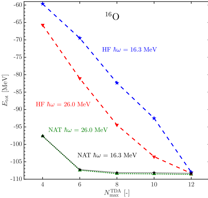
Fig. 3. The total energy E_{\text{tot}} of ^{16}\text{O} for different values of N_{\text{max}}^{\text{TDA}} . E_{\text{tot}} = E_{\text{HF}} + E_{\text{corr}} for the HF basis (HF) and E_{\text{tot}} = E_{\text{NAT}} + E_{\text{corr}} for the natural orbital basis (NAT). The energies are shown for two values of the HO frequency, \hbar\omega = 16.3 MeV and \hbar\omega = 26 MeV.
